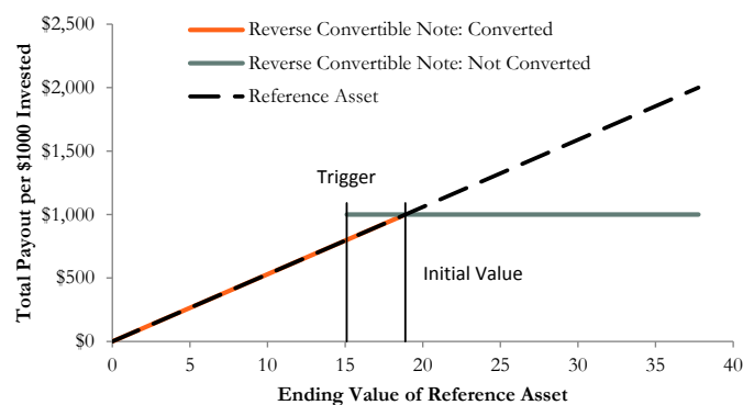
The payoff diagram shows the final payoff of this note given Pengrowth Energy Trust's stock price (horizontal axis). For comparison, the dashed line shows the payoff if you invested in Pengrowth Energy Trust's stock directly.
