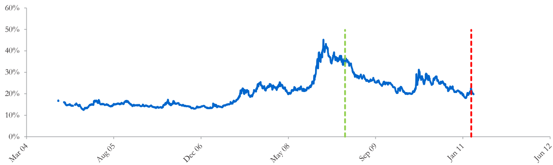
The annualized implied volatility of the S&P 500 Index on March 24, 2009 was 34.53%, meaning that options contracts on the S&P 500 Index were trading at prices that reflect an expected annual volatility of 34.53%. The higher the implied volatility, the larger the expected fluctuations of the S&P 500 Index level and of the Note's market value during the life of the Notes.
