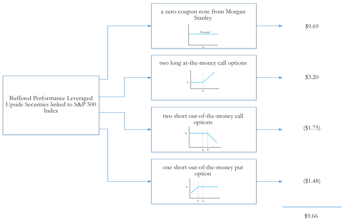
This note can be decomposed into different components, and each component can be valued separately. The chart above shows the value of each component of this Buffered Performance Leveraged Upside Security.
