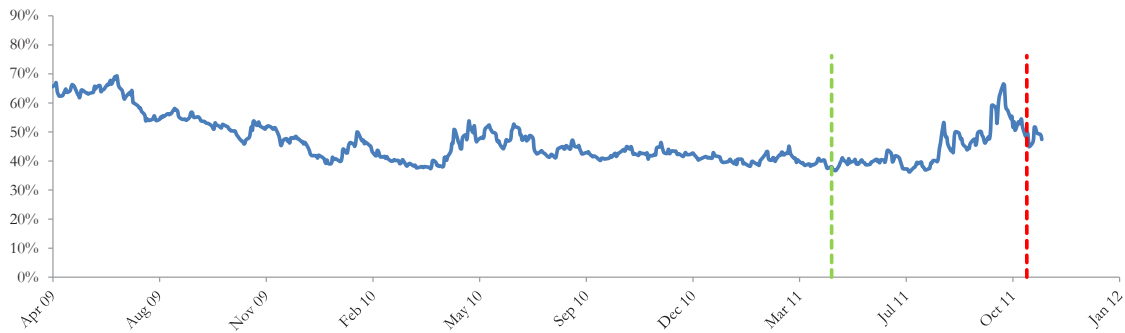
The annualized implied volatility of Freeport-McMoRan Copper & Gold, Inc.'s stock on April 25, 2011 was 38.01%, meaning that options contracts on Freeport-McMoRan Copper & Gold, Inc.'s stock were trading at prices that reflect an expected annual volatility of 38.01%. The higher the implied volatility, the larger the expected fluctuations of Freeport-McMoRan Copper & Gold, Inc.'s stock price and of the Note's market value during the life of the Notes.
