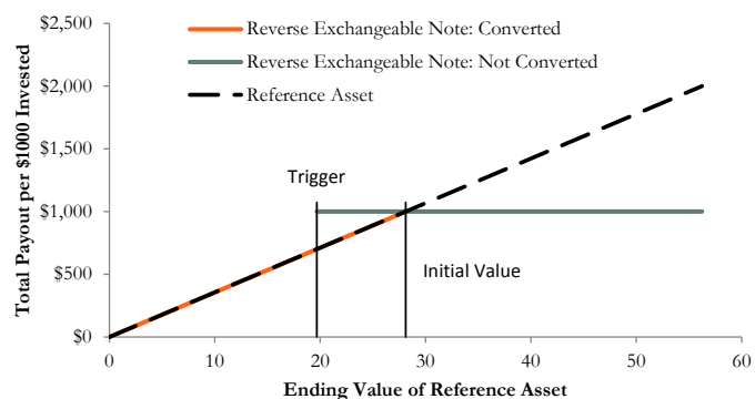
The payoff diagram shows the final payoff of this note given Ternium S.A.'s stock price (horizontal axis). For comparison, the dashed line shows the payoff if you invested in Ternium S.A.'s stock directly.
